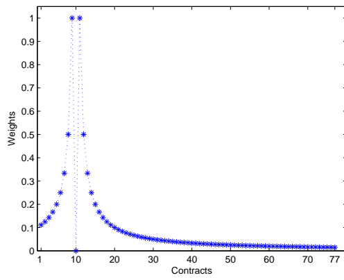
(c) w_{10}
