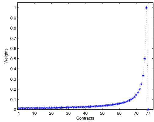
(f) w_{77}
