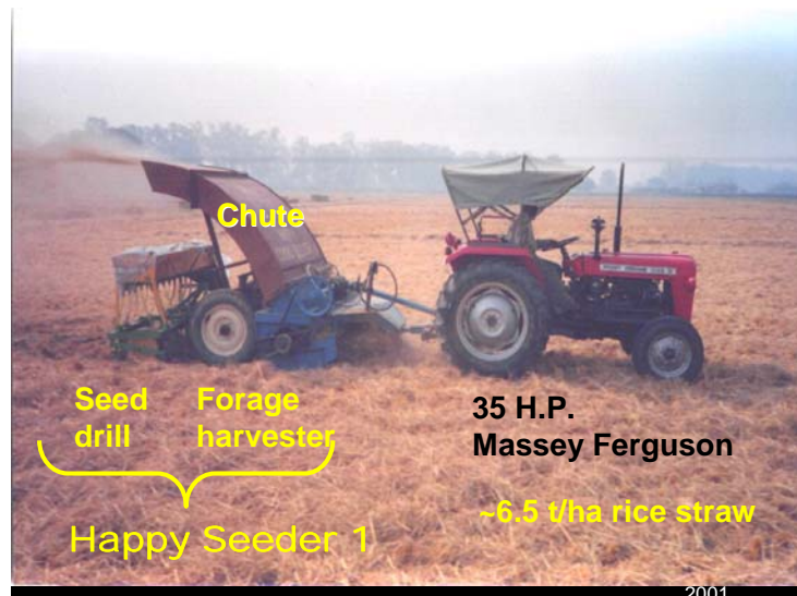
Figure 3. The Original Happy Seeder (photo J. Blackwell)
