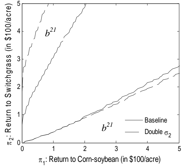
Figure 7a. Return volatility (under GBM): conversion boundary
