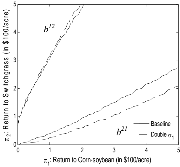
Figure 7a. Return volatility (under GBM): conversion boundary
