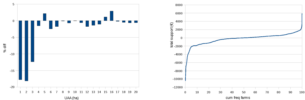
(a) size effects (cum nFarms by size)
