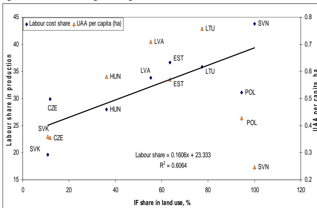
Figure 5: Labour content in agricultural goods and farm structure in CEE
