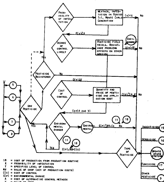
FIGURE 5. PESTICIDE SUBROUTINE
