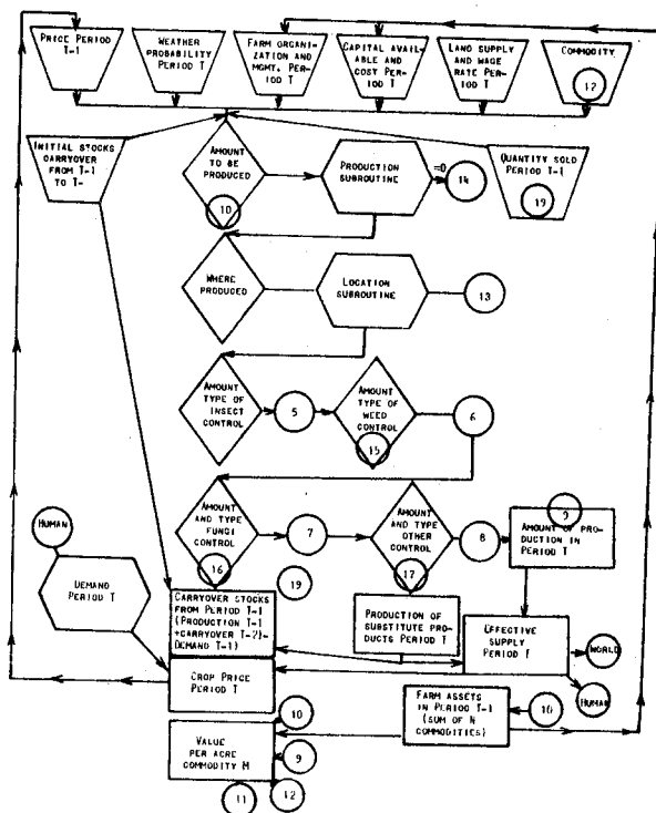
FIGURE 4. AGRICULTURE SUBSYSTEM
