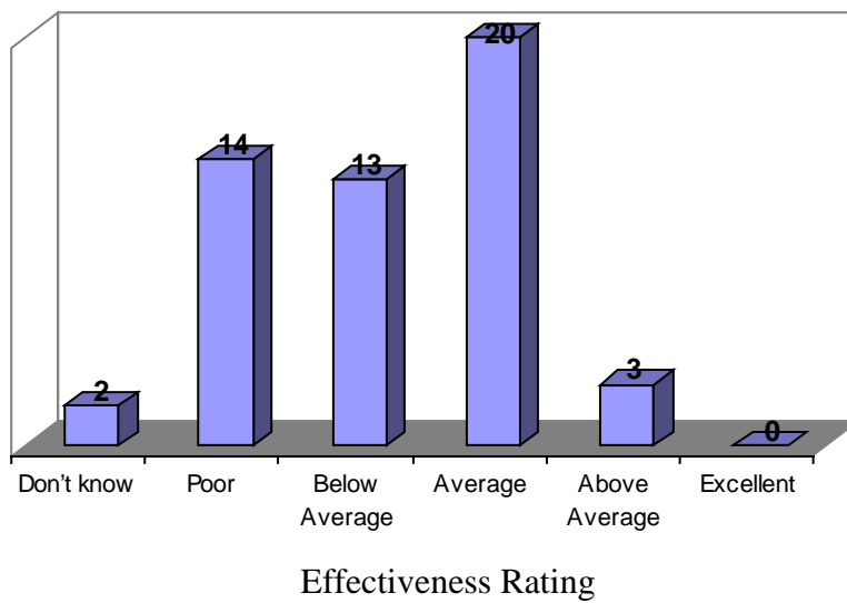
Figure 10 Frequency of Effectiveness Ratings for Method 12
