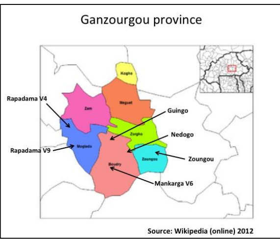
Figure A2. Distribution of selected villages in the north bio-area, provinces of: Banwa, Mouhoun, Sanguie, Bazega, and Ganzourgou.
