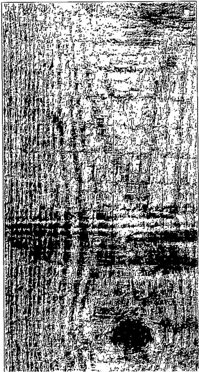
A check in 1 by 6 inch lumber resulting from the uneven drying caused by an excessively wide sticker. Narrow stickers, from 1\frac{1}{4} to 2 inches in width, permit better drying of the wood they cover.
