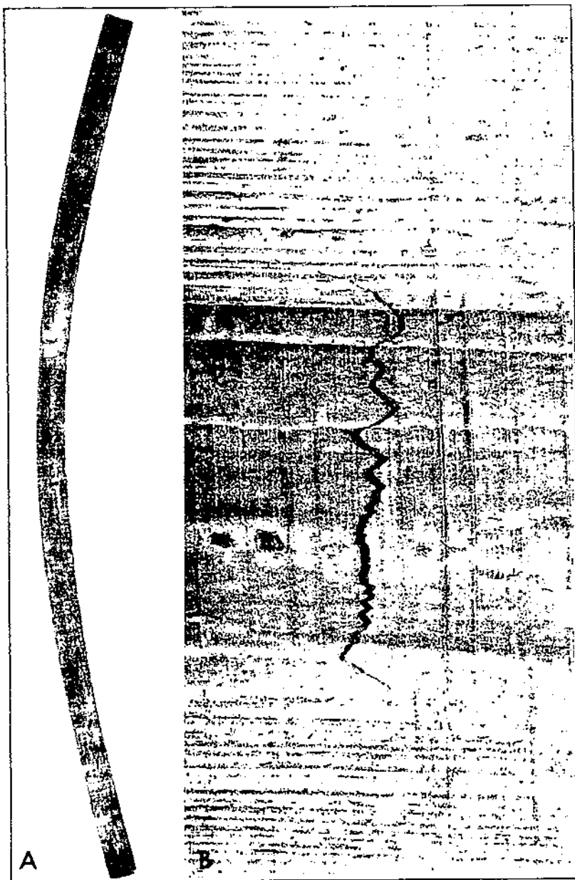
A. Crack in 1 by 1 inch kiln-dried southern yellow pine, caused by the longitudinal shrinkage of compression wood during drying. B. A typical tension failure in southern yellow pine caused by the longitudinal shrinkage of compression wood during seasoning.
